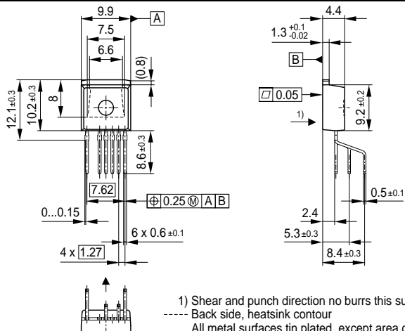
Figure 23 P-TO220-6-46 (Isodrain I2Pak Package)
