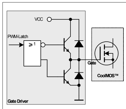
Figure 10 Gate Driver
