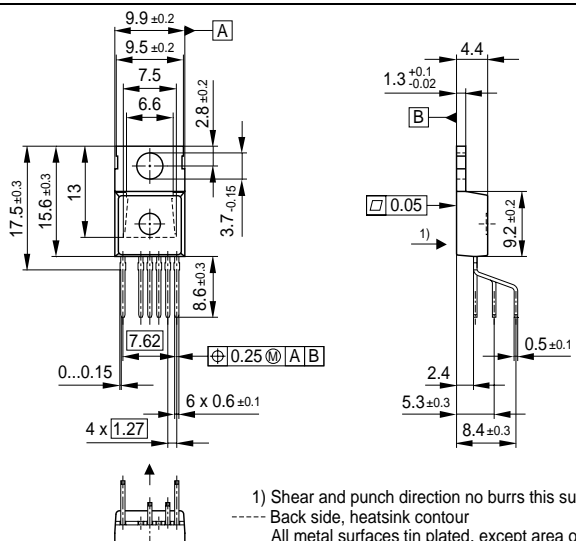
Figure 24 P-TO220-6-47 (Isodrain Package)
